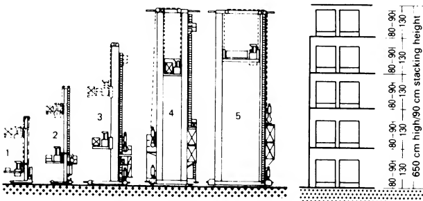
9 Handling machines
